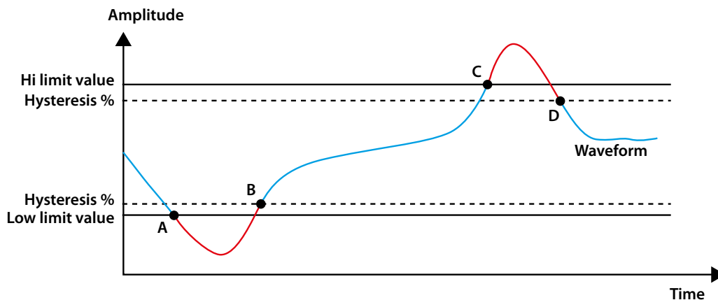
Fig. 3-57 Alarm Example
